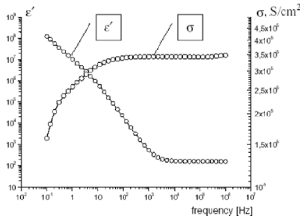
Fig 9: Electrodynamic characteristics of non-activated distilled water at temperature 20°C.
